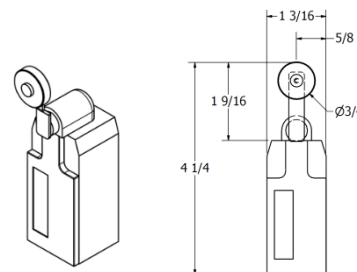
99-267 – Washdown Roller Type
