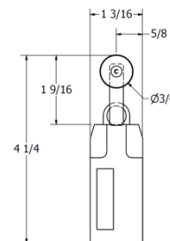
99-267 – Washdown Roller Type
