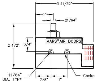
99-012 - Plunger Type
