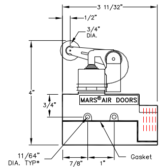
99-014 – Combination Plunger/Roller Type
