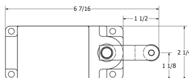
99-015 – Washdown Roller Type
